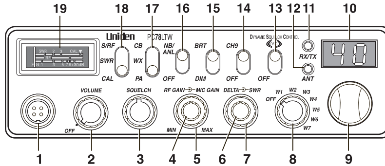
FRONT VIEW - PC781TW BACKLIT PANEL
